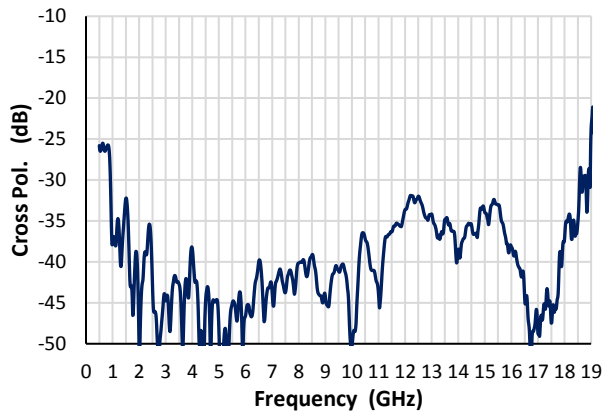
Cross Polarization
