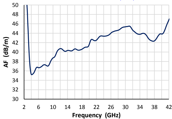
Antenna Factor (1m)
